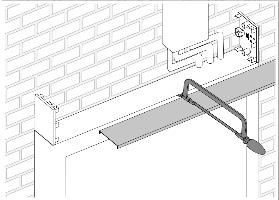
Fig. 47: Cutting covers
