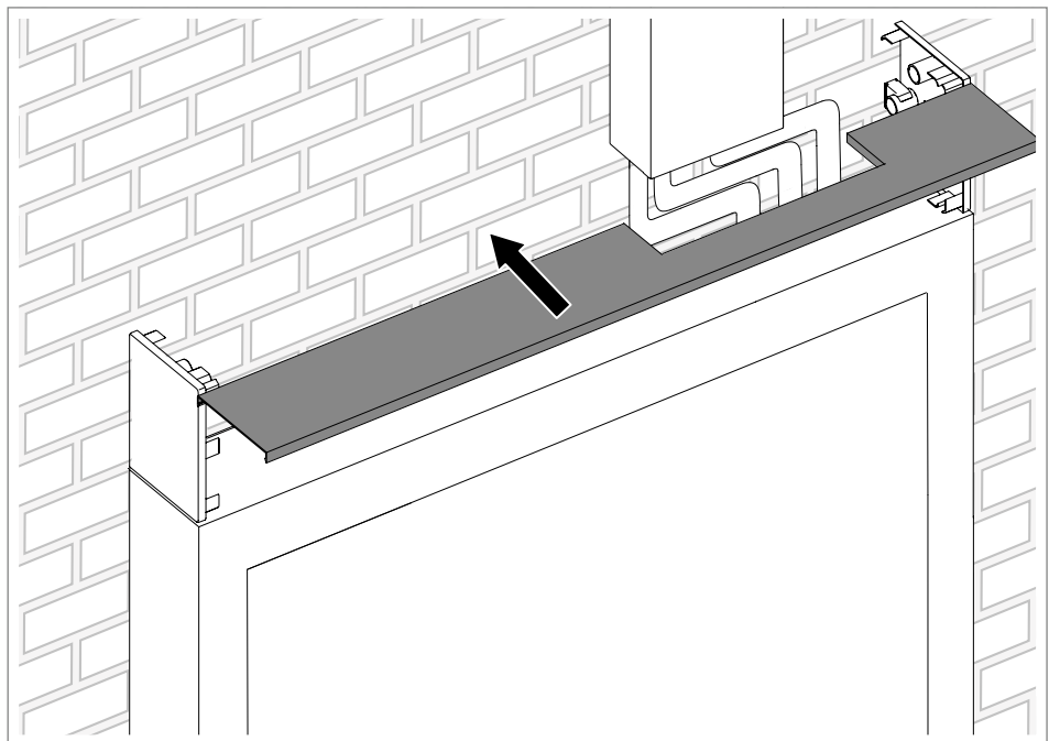
Fig. 48: Installing covers
