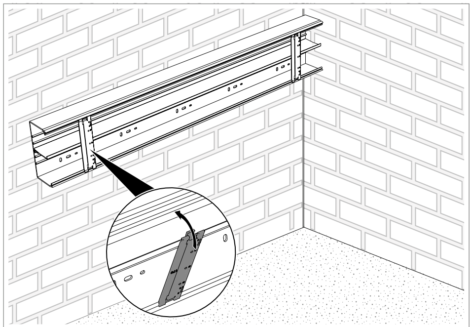
Fig. 13: Mounting cover clips
