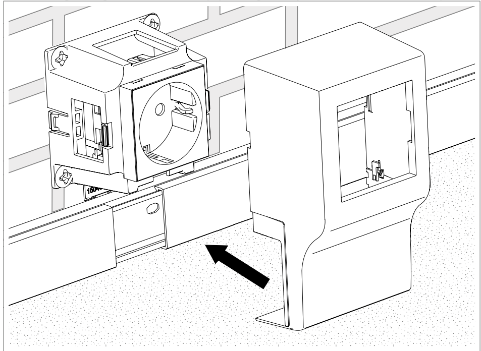
Fig. 31: Mounting the cover
