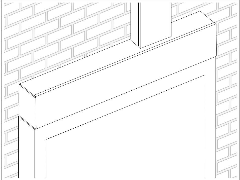
Fig. 51: Universal trunking
