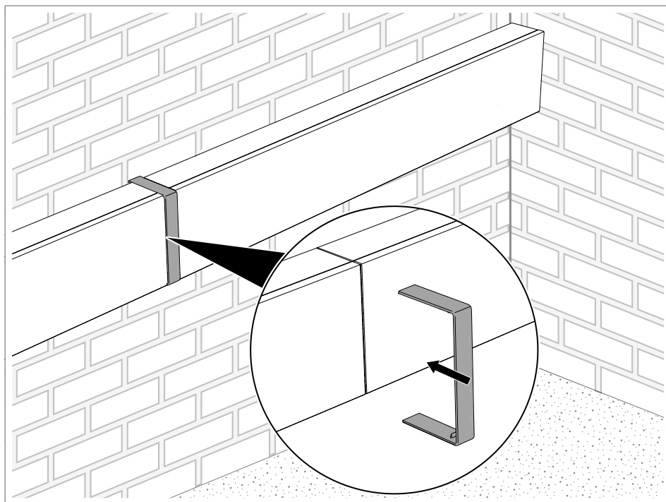
Fig. 43: Mounting the joint cover
