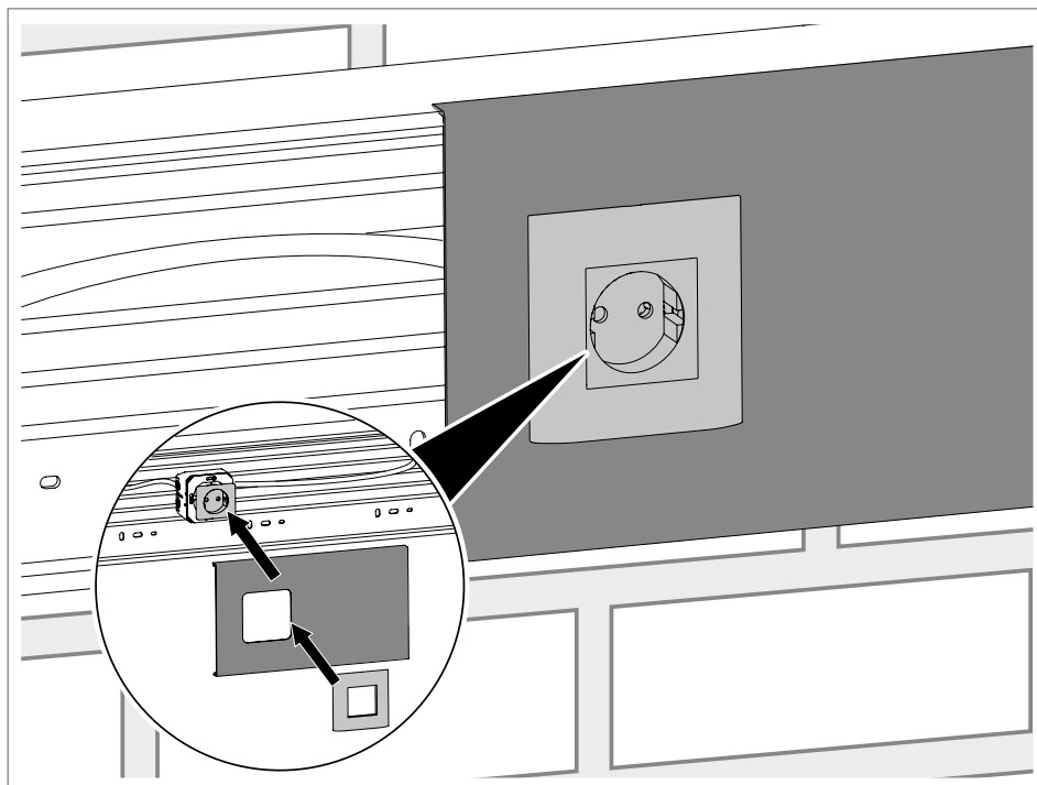
Fig. 20: Screwing on the device installation socket for Schuko sockets
