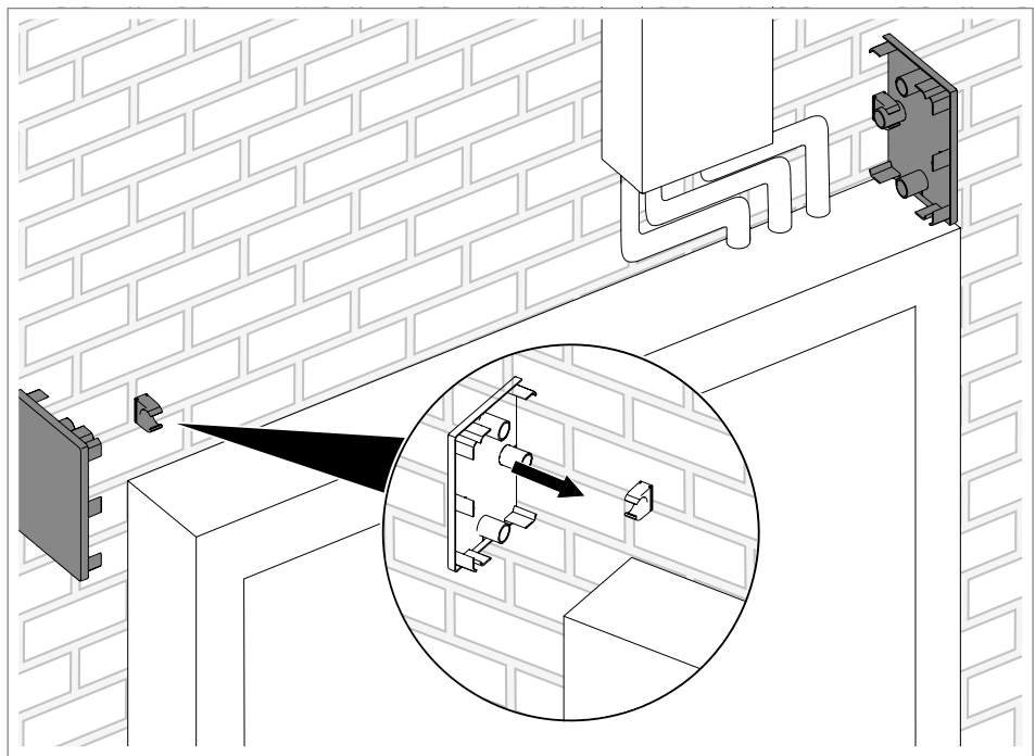
Fig. 46: Mounting end pieces
