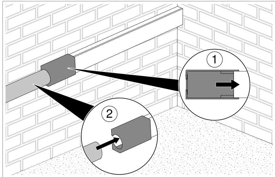
Fig. 15: Mounting the pipe adapter
