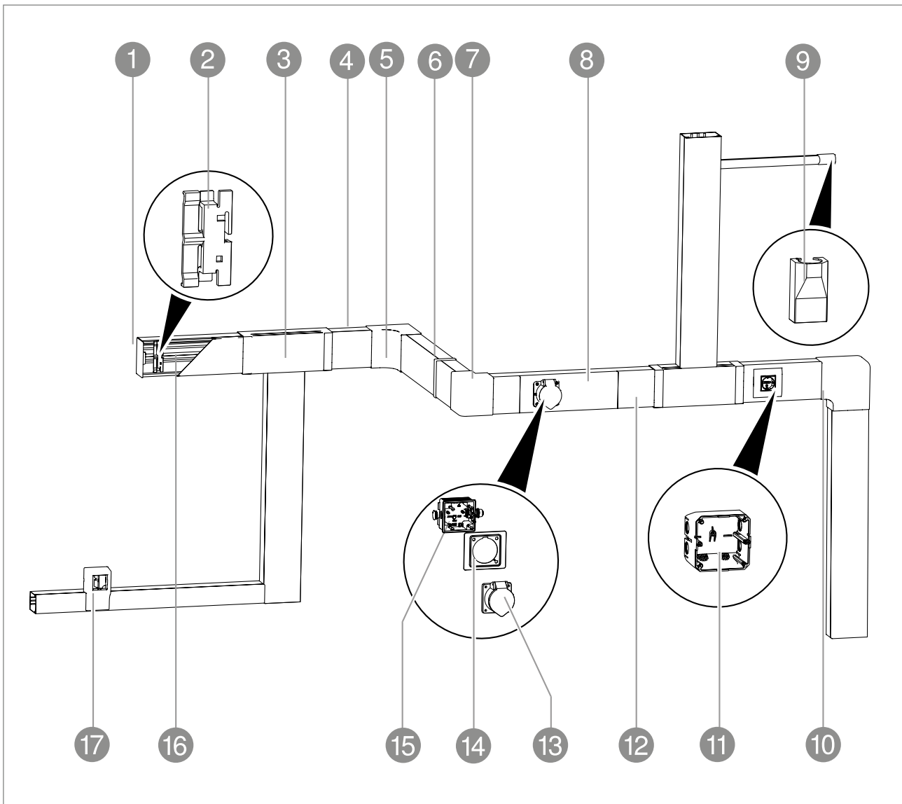
Fig. 6: Overview, WDK cable trunking system
