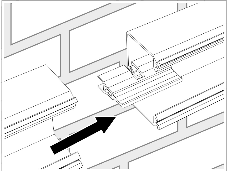
Fig. 10: Mounting the WDK cable trunking
