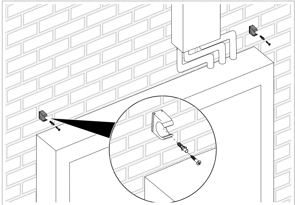
Fig. 45: Mounting fastening clips
