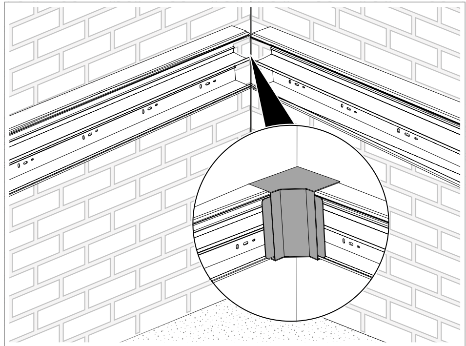
Fig. 33: Mounting the internal corner cover
