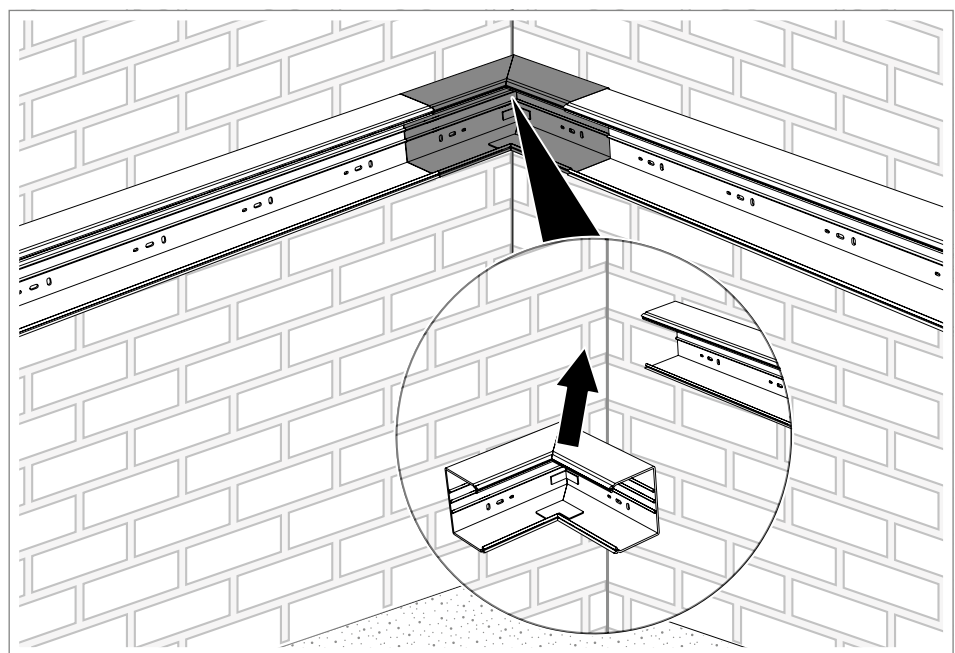
Fig. 34: Mounting an internal corner
