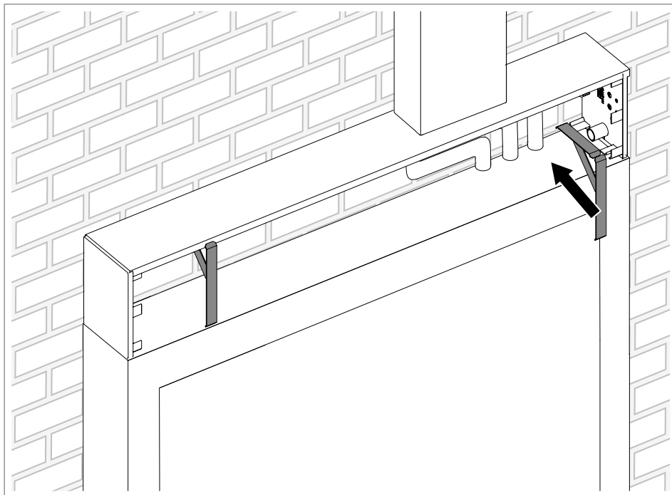
Fig. 49: Mounting cover clips
