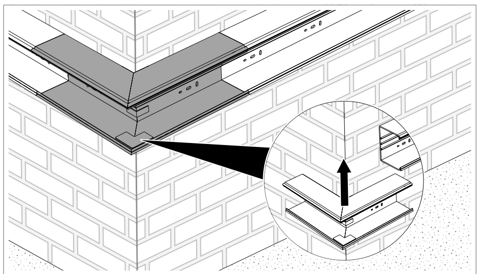
Fig. 36: Mounting an external corner
