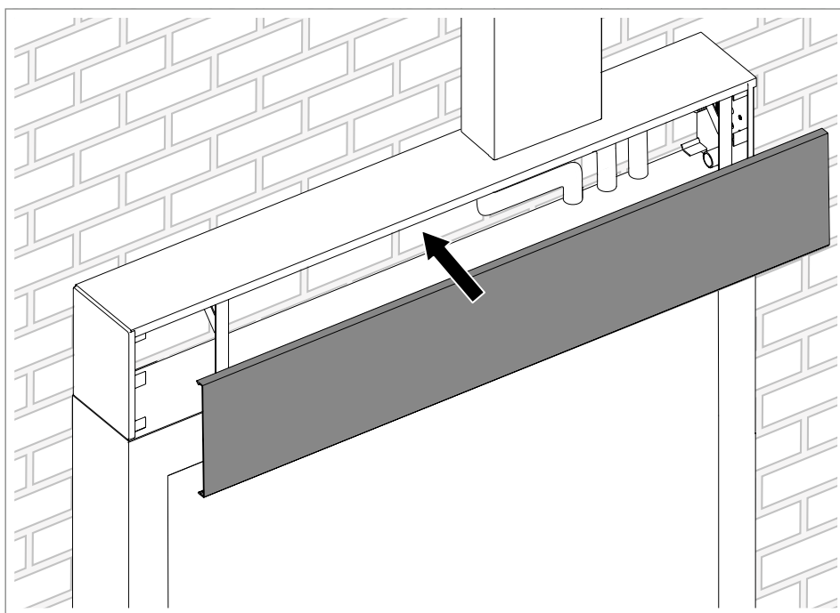
Fig. 50: Mounting the front cover
