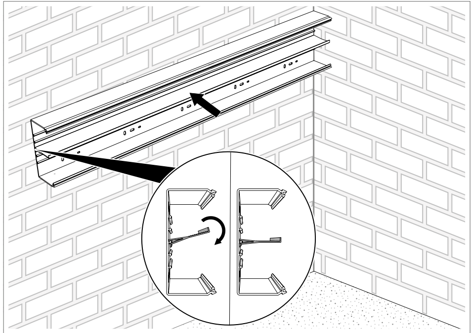
Fig. 12: Mounting the partition
